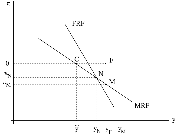
Figure 2: Nash Non-cooperative Equilibrium
