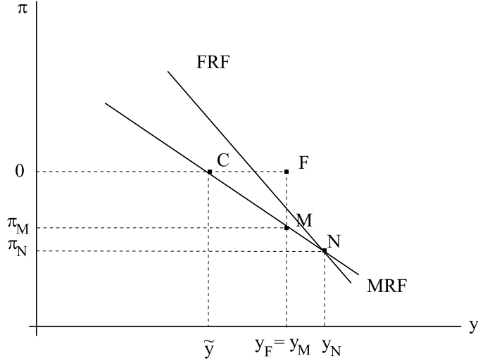
Figure 3: Extreme Nash Equilibrium with Fiscal Non-cooperation
