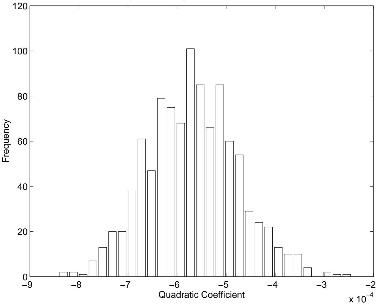
Sample Frequency Plot of 1,000 Simulations
