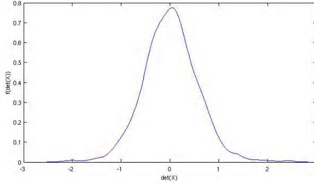
Figure 1: Kernel density estimate of the density of \det(\mathbf{X}) = \Delta X .
