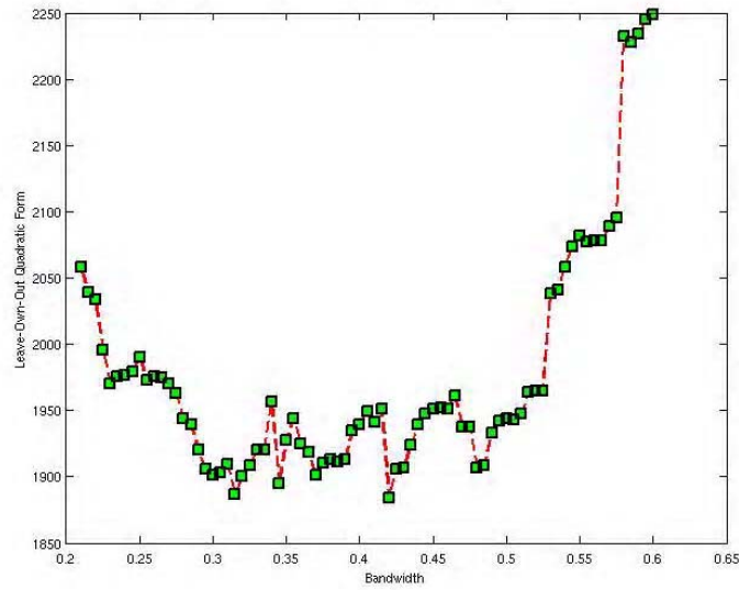
Figure 2: Leave-own-out ‘IV’ quadratic form for different bandwidth values – Column 7, Table 5 specification.
