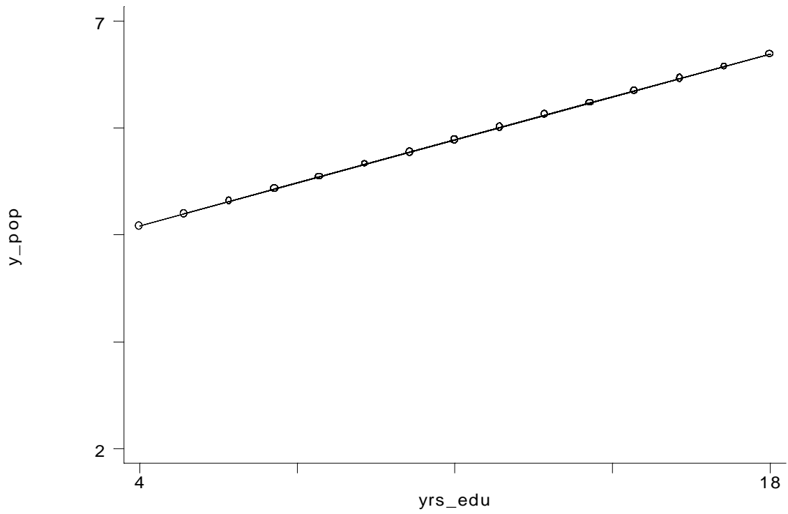
Figure 2: Sample 1 Regression Line (OLS Random sample n=30 for State 53, Females, 1995)
