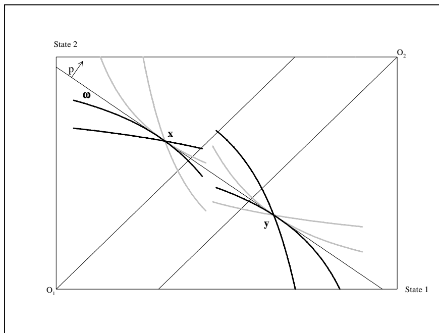
Figure 3: Multiple Equilibria
