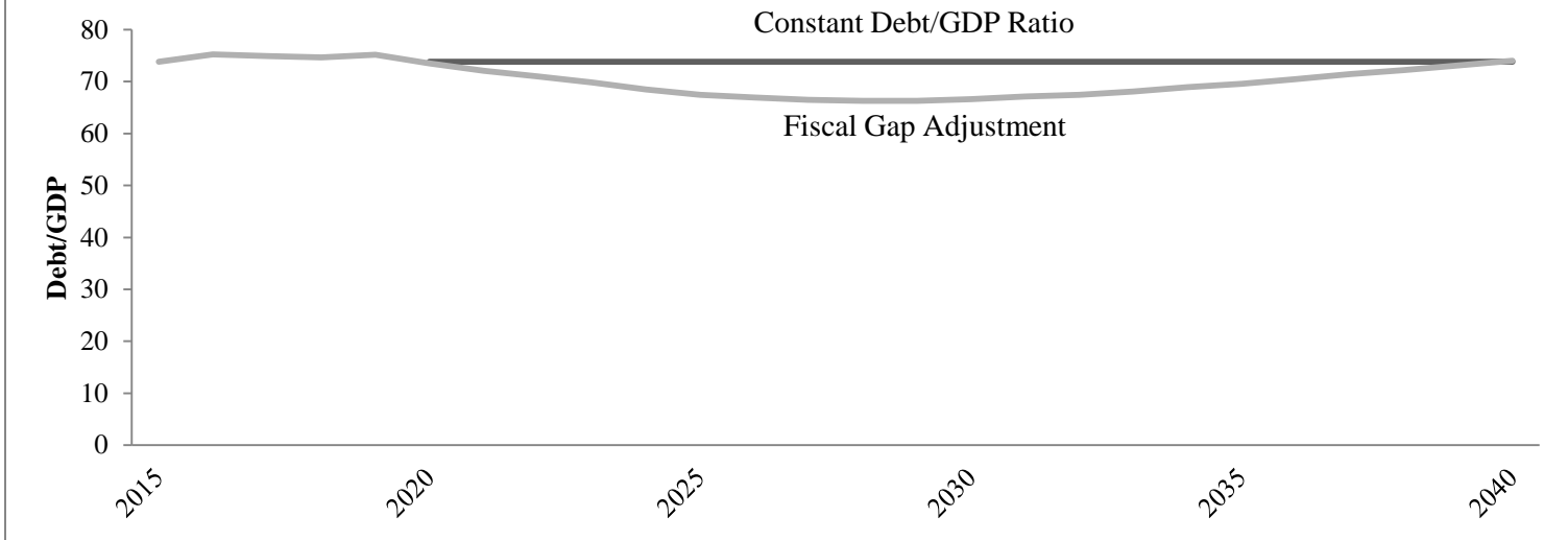
Figure 7. Two Ways to Obtain a 74.0% Debt/GDP Ratio by 2040
