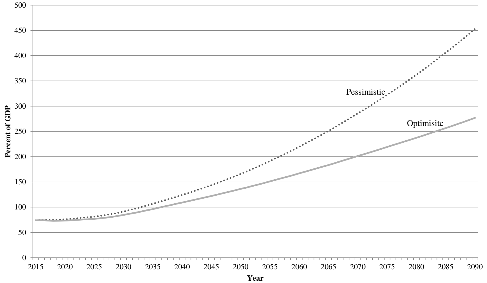
Figure 6. Alternative Projections of the National Debt, 2015-2090
